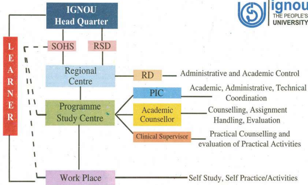
Fig. 4: Implementation Model
